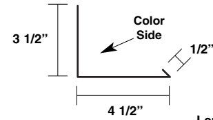
Commercial Rake Flashing Item #: 38386
