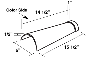
Commercial Ridge / Hip Flashing* Item #: 38419
