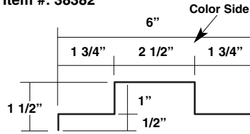
Counter Flashing Item #: 38382
