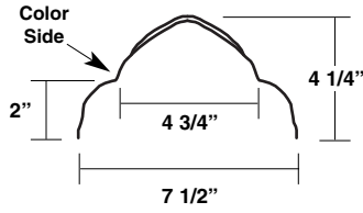
Contoured Rake Flashing Item #: 38394
