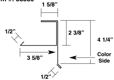
Commercial Rake Flashing Item #: 38386
