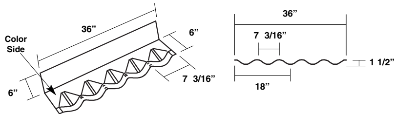
Contoured Hi-Side Tie-In Flashing Item #: 38396
